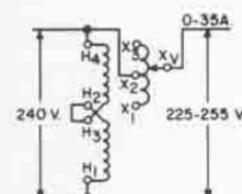
LIMITED RANGE TRANSFORMER
