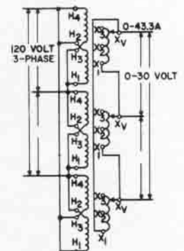
LOW VOLTAGE TRANSFORMER
