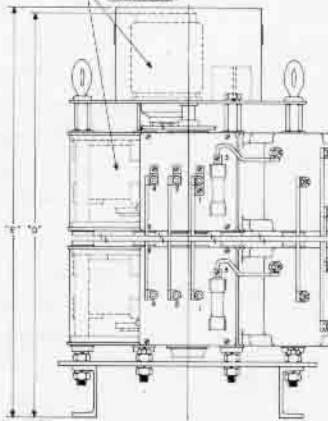
4-GANG TO 9-GANG MOTOR DRIVEN
